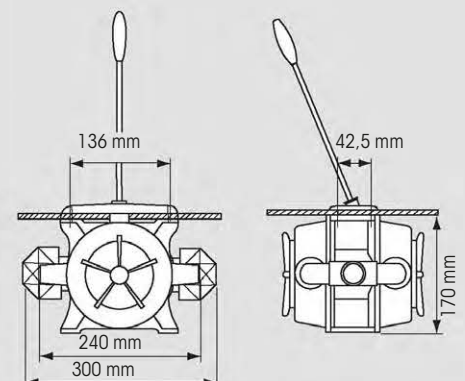
Double action with watertight gasket
