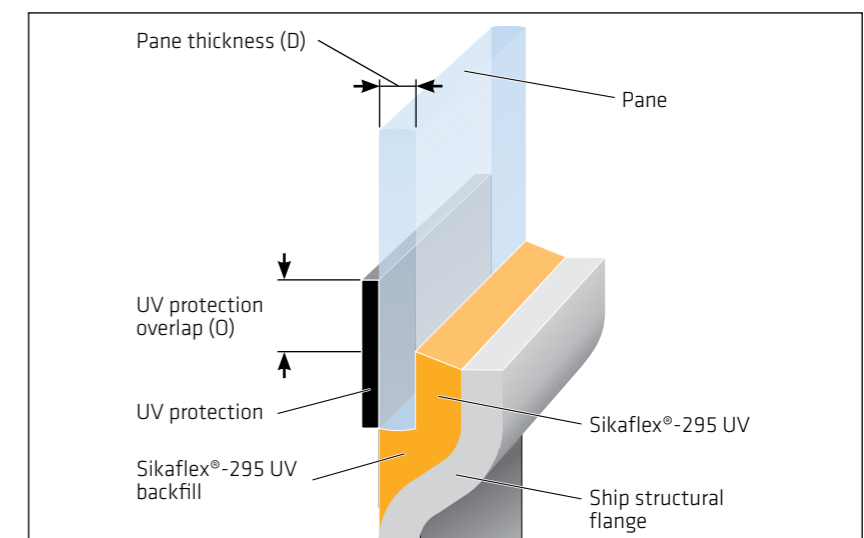
Fig. 98 Bonding a decorative panel vertically
