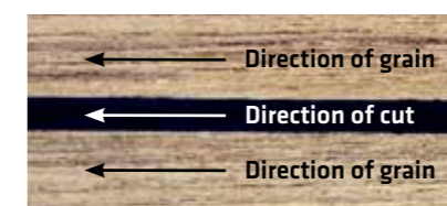
Fig. 59 Always ensure that the direction of cut is with the grain to avoid 'digging-in' damage to the sides of the planks
