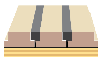
Fig. 50 Typical prefabricated teak deck profiles
