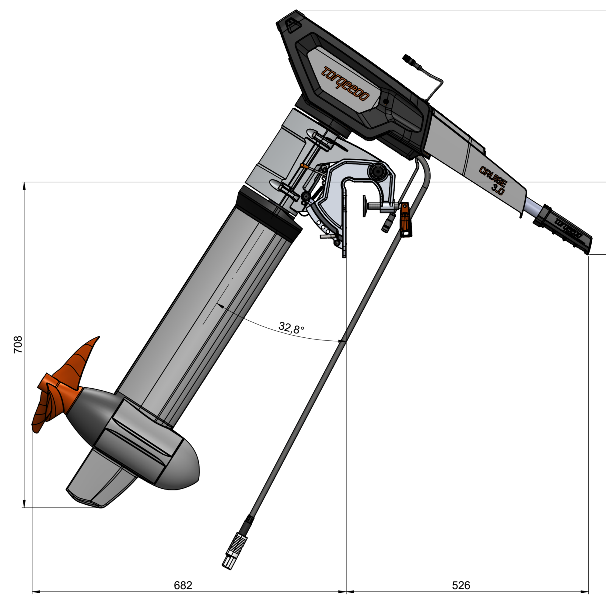
Tilt Position 2 Tilt position 2 Cruise 3/6 TL
