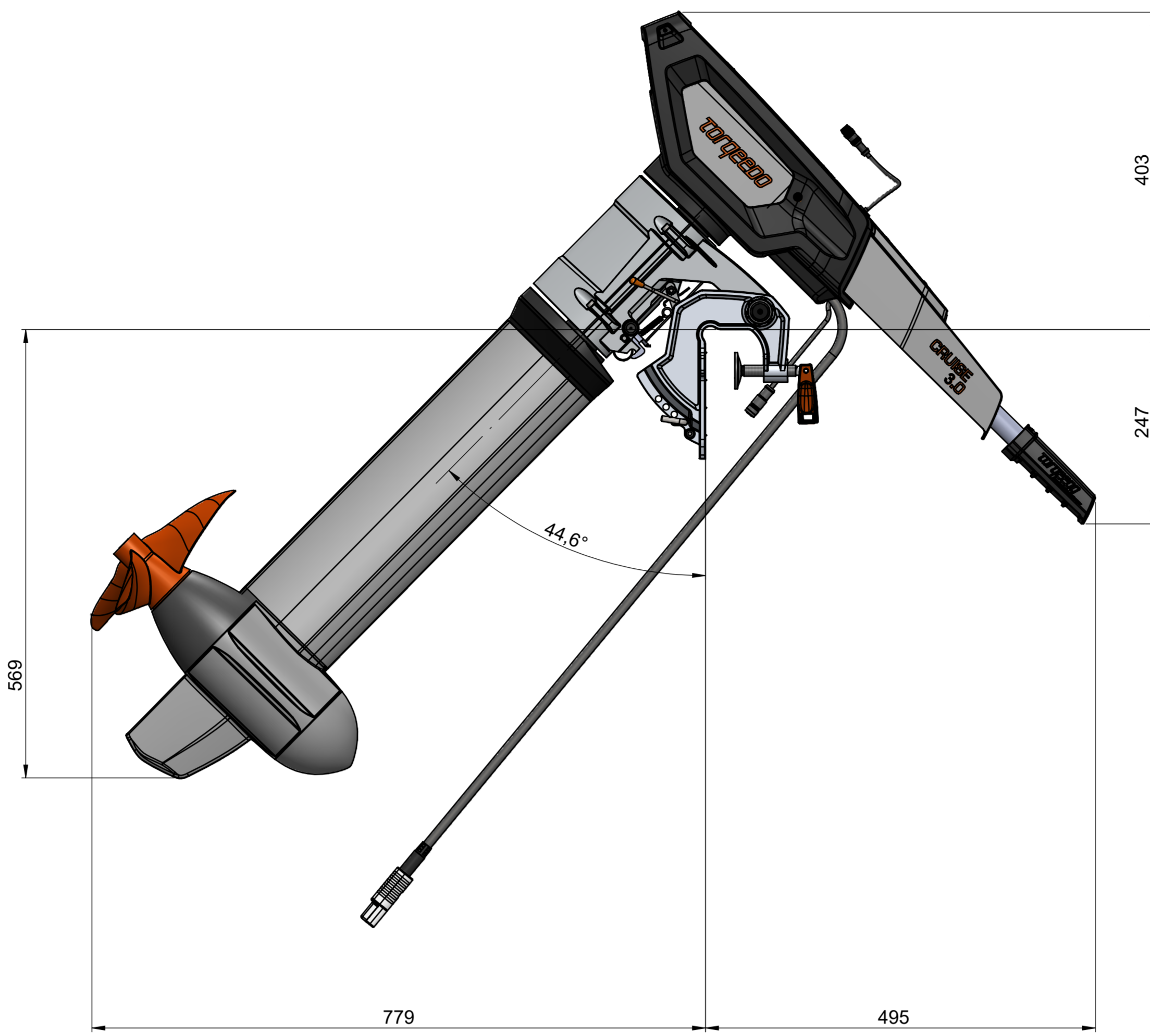
Tilt Position 3 Tilt position 3 Cruise 3/6 TL
